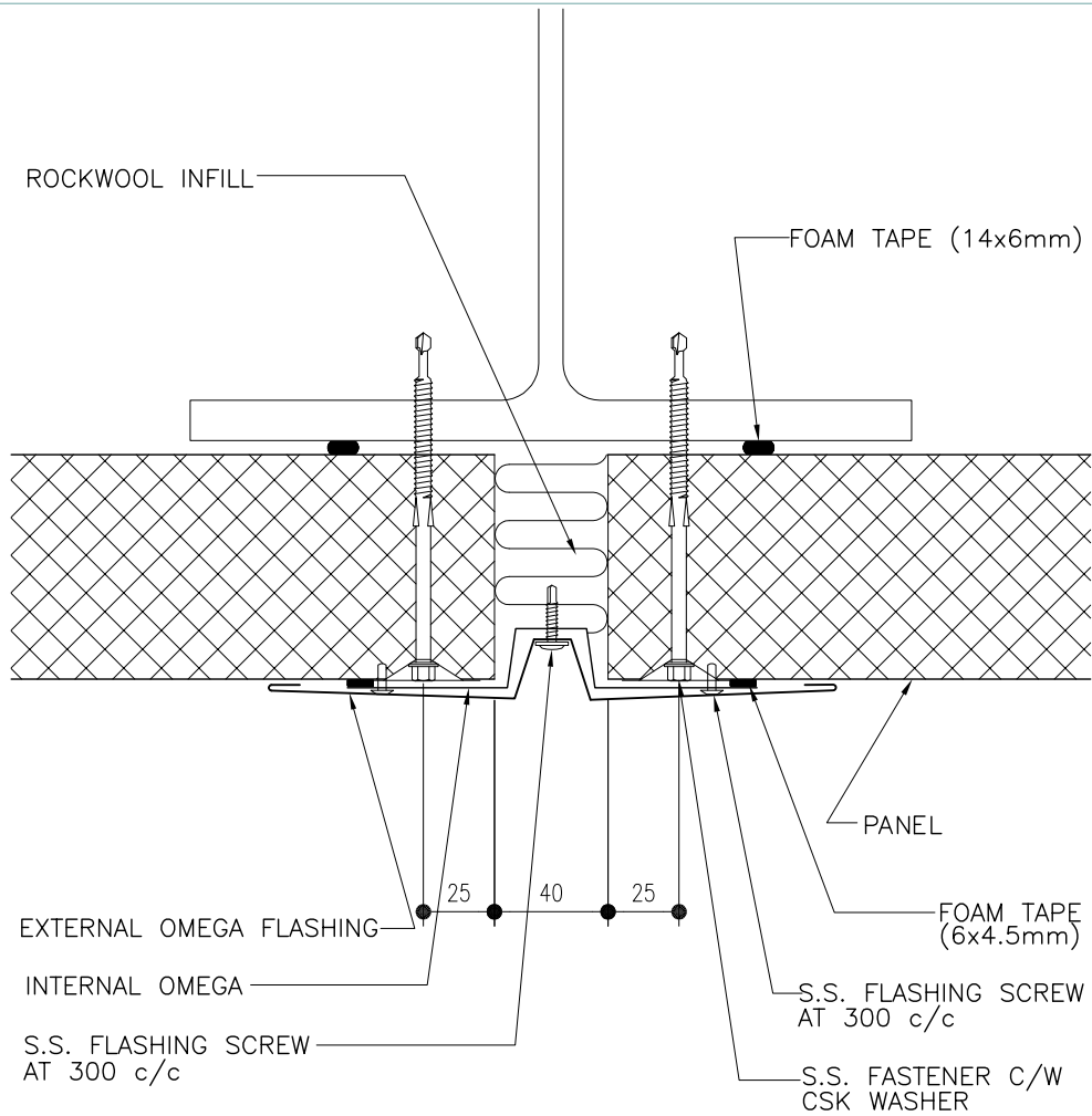
VERTICAL JOINT OMEGA DETAIL
